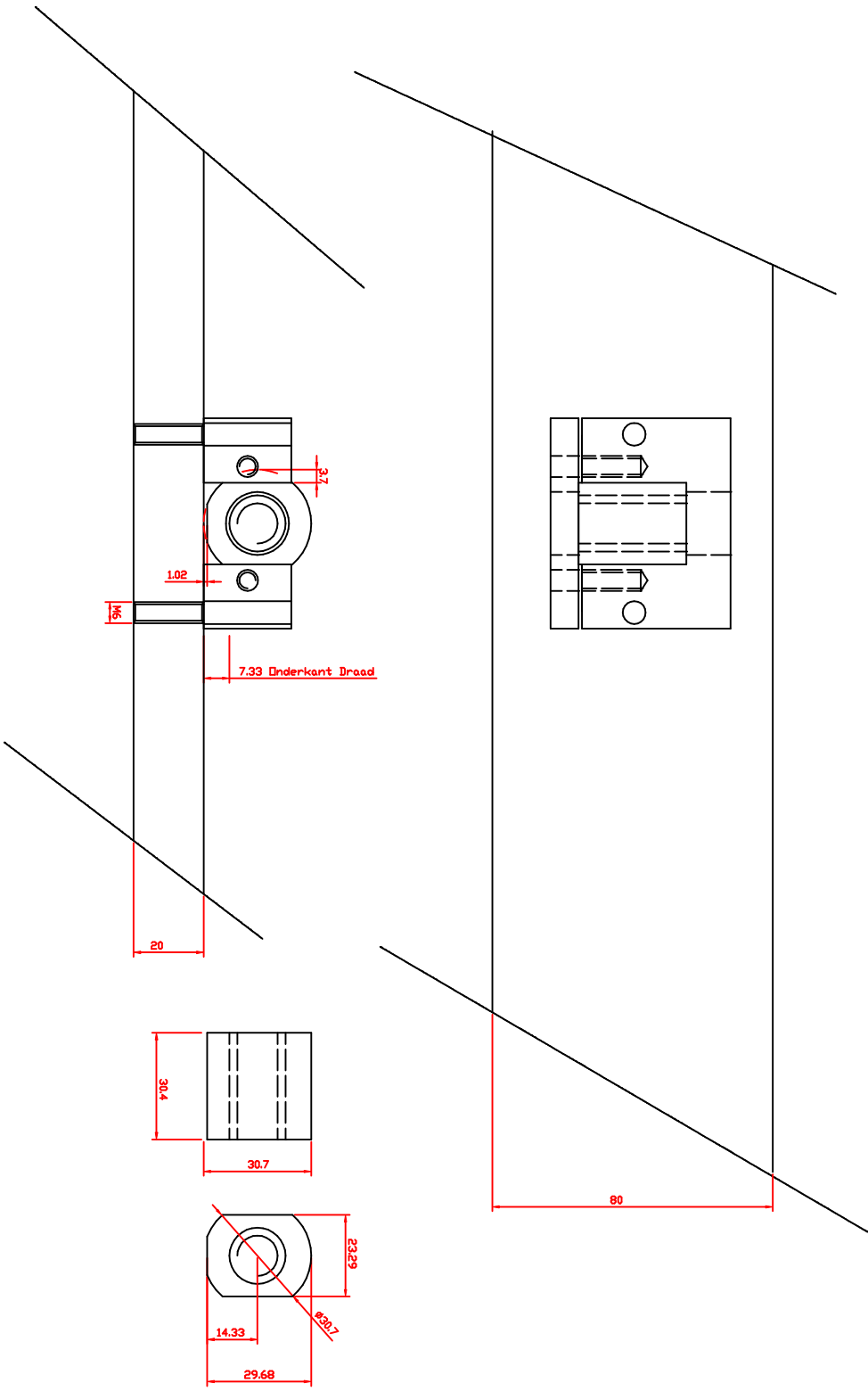
Trapezium nut holder for centering to X as J.Stinissen 07-12-2000
